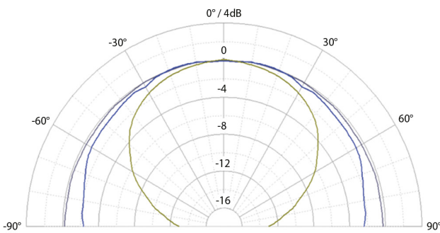
Polar pattern (1m)
